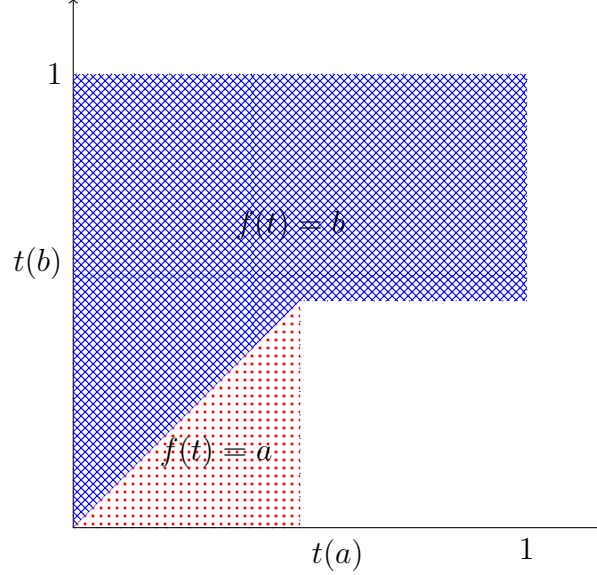
Figure 4.1: An example with two alternatives
