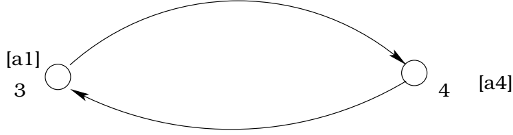
Figure 6.9: Cycle in stage 2 of the FPTTC mechanism
