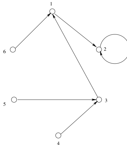
Figure 6.3: Cycle in Step 1 of the TTC mechanism
