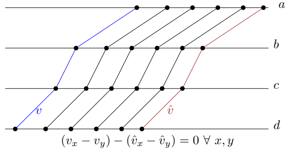
Figure 1.3: A quasilinear preference
