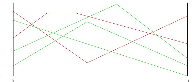
Figure 6.1: Examples of single-peaked preferences
