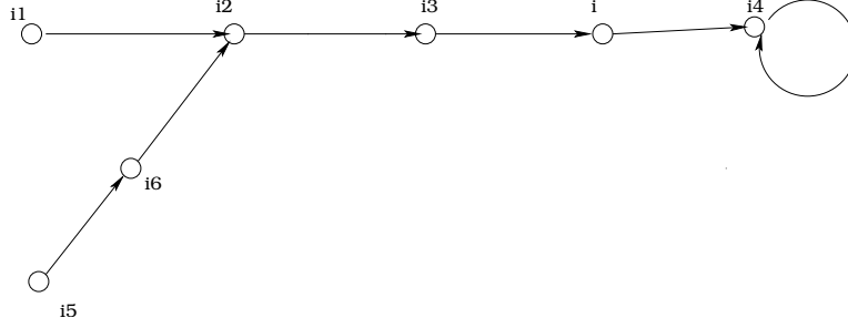
Figure 6.7: i -Paths in a Step
