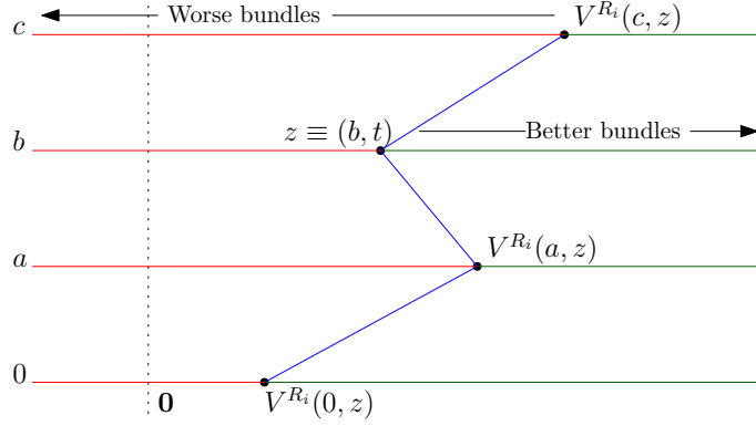
Figure 1.2: Valuation at a preference
