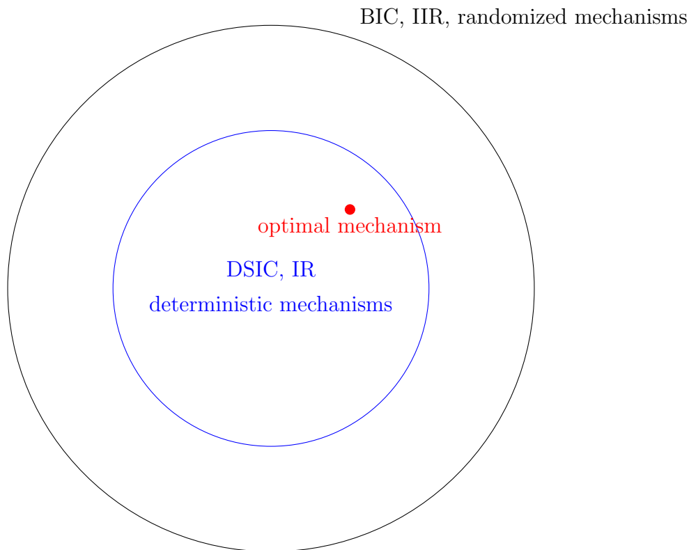
Figure 3.6: Optimal mechanism is DSIC, IR, and deterministic
