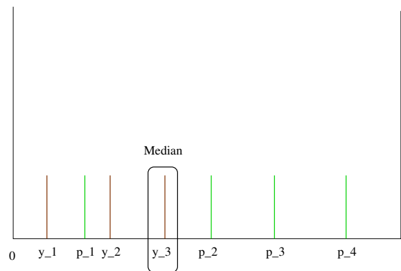
Figure 6.2: Phantom voters and the median voter
