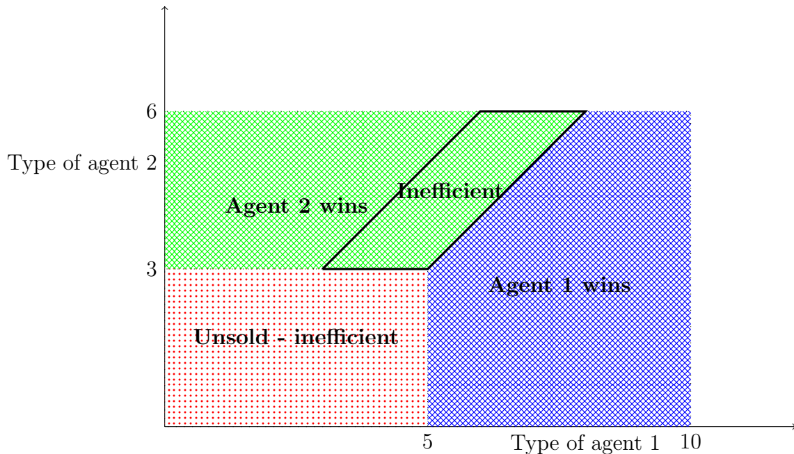
Figure 3.7: Inefficiency of optimal mechanism
