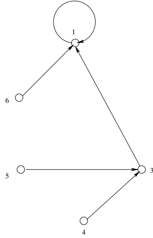
Figure 6.4: Cycle in Step 2 of the TTC mechanism
