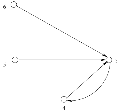
Figure 6.5: Cycle in Step 3 of the TTC mechanism
