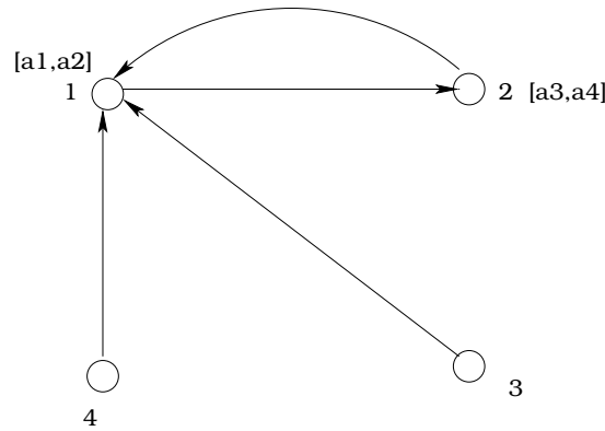
Figure 6.8: Cycle in stage 1 of the FPTTC mechanism
