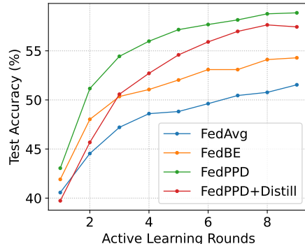
Figure 3: Federated Active Learning on CIFAR-10 dataset. Note: FedAvg+SWAG performed almost similarly to FedAvg on this task as well so we skip it from the plot.
