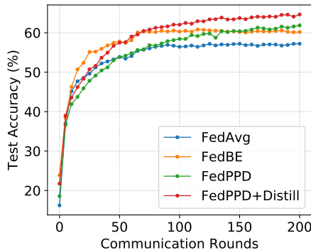
Figure 2: Convergence of all the methods on CIFAR-10 dataset
