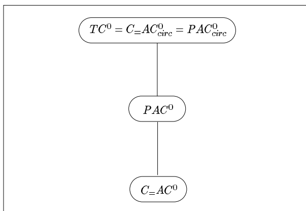
Figure 1: Logspace-uniform setting ([ABL98] shows these all coincide)
