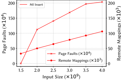
Fig. 5. Scaling of page faults and remote mapping events in HT-UVM
