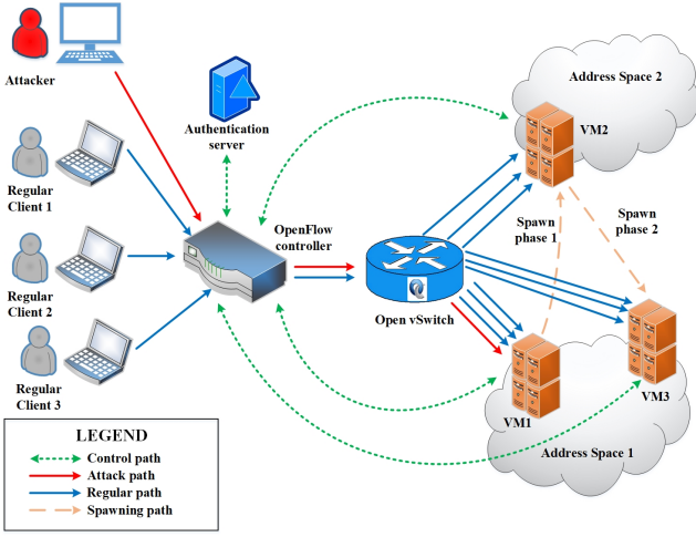
Fig. 1: The cloud system model for Whack-a-Mole
