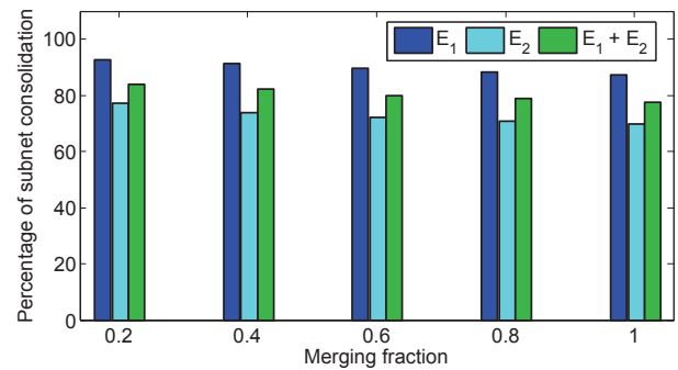
Fig. 7. Percentage of entries reduced after the merge-split based coalition game.
