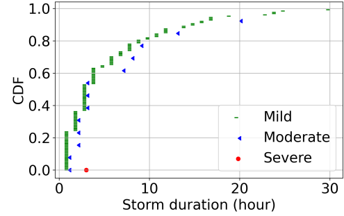
Fig. 2: Distribution of storm duration.
