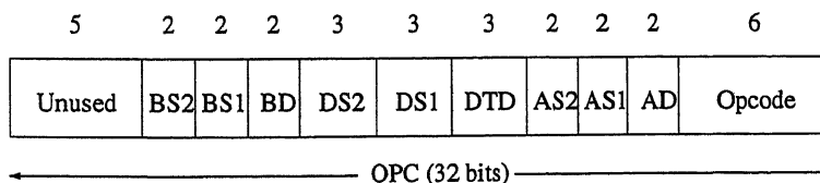
Figure 5: Instruction Encoding
