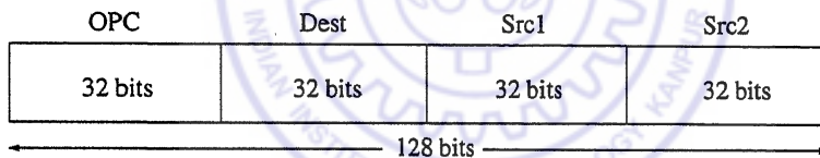
Figure 4: Instruction Format
