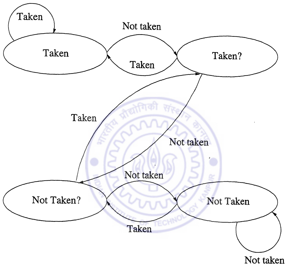
Figure 7: State Diagram for a 2-bit Branch Prediction Scheme
