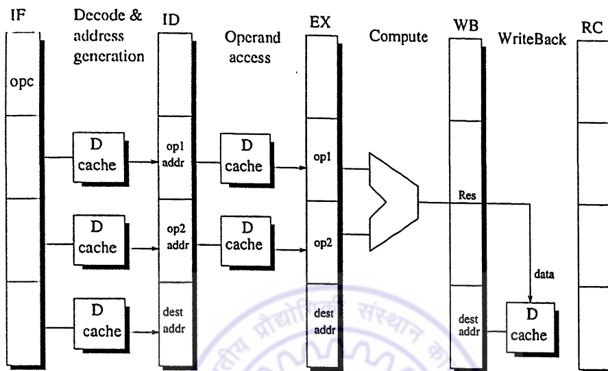
Figure 6: Processor Pipeline
