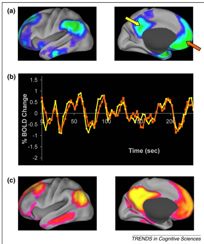
Figure 2. Performance of a wide variety of tasks has called attention to a group of brain areas (a) that decrease their activity during task performance (data adapted from [31]). These areas are often referred to as the brain's DMN [32]. If one records the spontaneous fMRI BOLD signal activity in these areas in the resting state (arrows, a) what emerges is a remarkable similarity in the behavior of the signals between areas (b), a phenomenon originally described by Biswal and colleagues in the somatomotor cortex [147] and later in the DMN by Greicius and colleagues [38]. Using these fluctuations to analyze the network as a whole reveals a level of functional organization (c) that parallels that seen in the task-related activity decreases (a).
