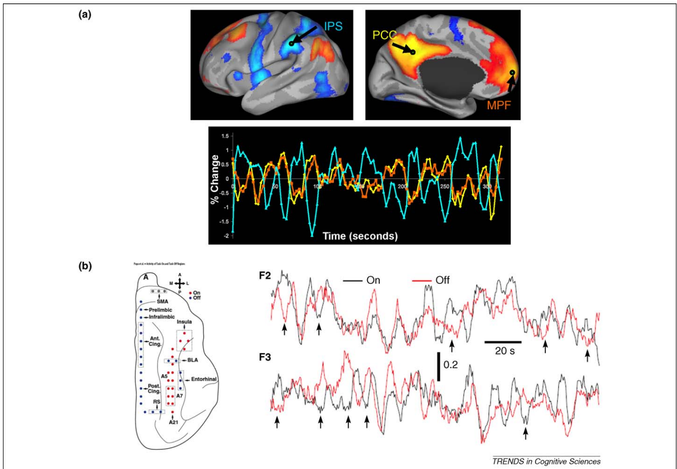
Figure 5. A. Intrinsically defined anti-correlated networks in the awake human observed with resting state fMRI. Positive nodes are significantly correlated with seed regions involved in focused attention and working memory (attention-positive seeds), and significantly anti-correlated with seed regions routinely deactivated during attention-demanding cognitive tasks (i.e. DMN). Negative nodes are significantly correlated with attention-negative seeds and significantly anti-correlated with attention-positive seeds. Reproduced, with permission, from [94]. B. Slow LFP power fluctuations in the awake cat reveal anti-correlated networks. These recordings were obtained from chronically implanted microelectrodes situated in the putative homolog of the DMN (midline blue electrodes) and regions thought to correspond to the attention-positive seeds in the human brain (blue). In these two recording epochs (F2 and F3) anticorrelations (arrows) alternated with periods of correlation between the two brain regions. Anticorrelations were present approximately 20% of the time. Reproduced, with permission, from [95]. This percentage dropped significantly during REM and slow wave sleep (personal communication, Denis Pare).
